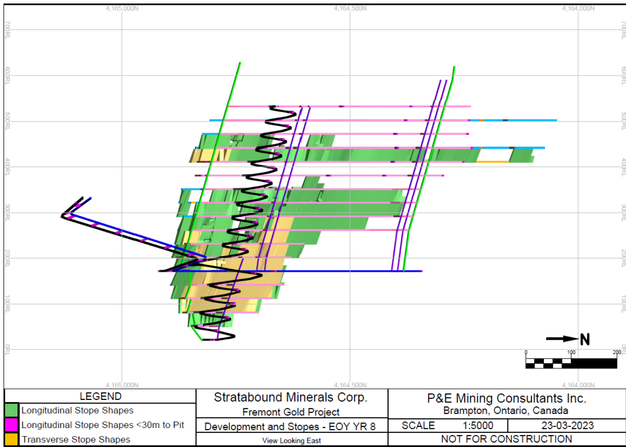
FIGURE 16.17 UNDERGROUND WORKINGS AS OF YEAR 8
