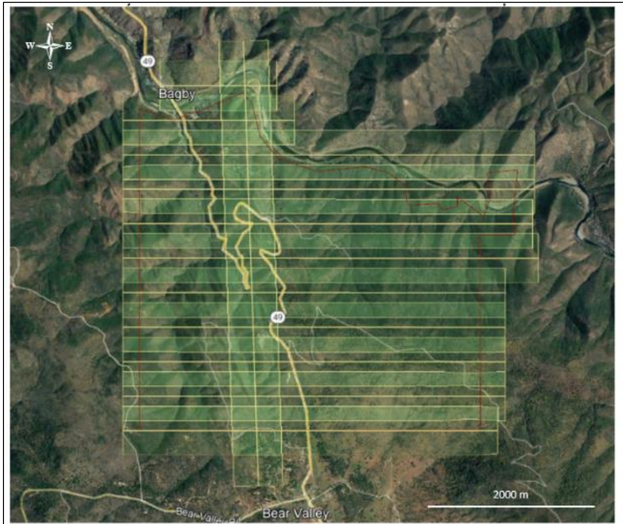
FIGURE 9.4 FREMONT PROPERTY LIDAR™ SURVEY COVERAGE
