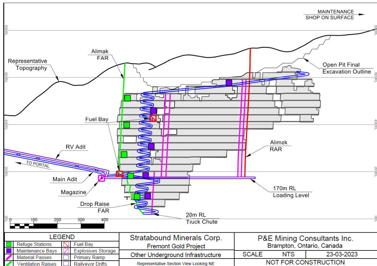
FIGURE 16.13 UNDERGROUND INFRASTRUCTURE
