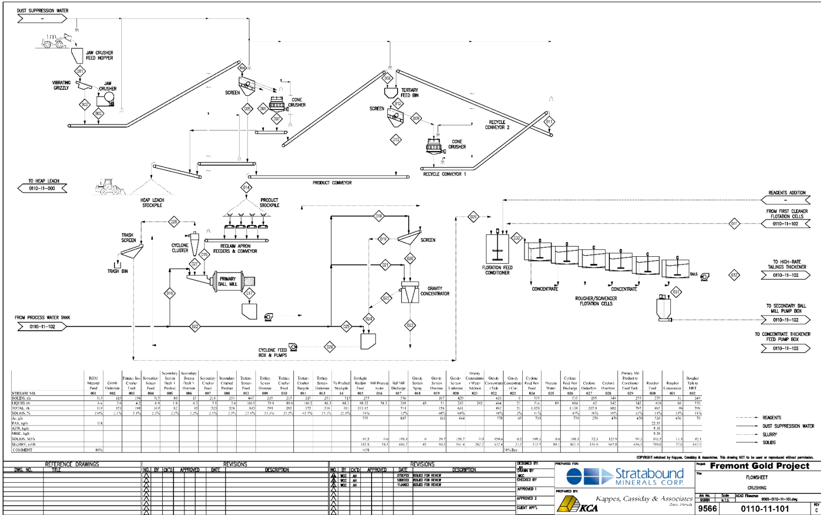
FIGURE 17.2 FLOTATION CONCENTRATOR FLOWSHEET 1
