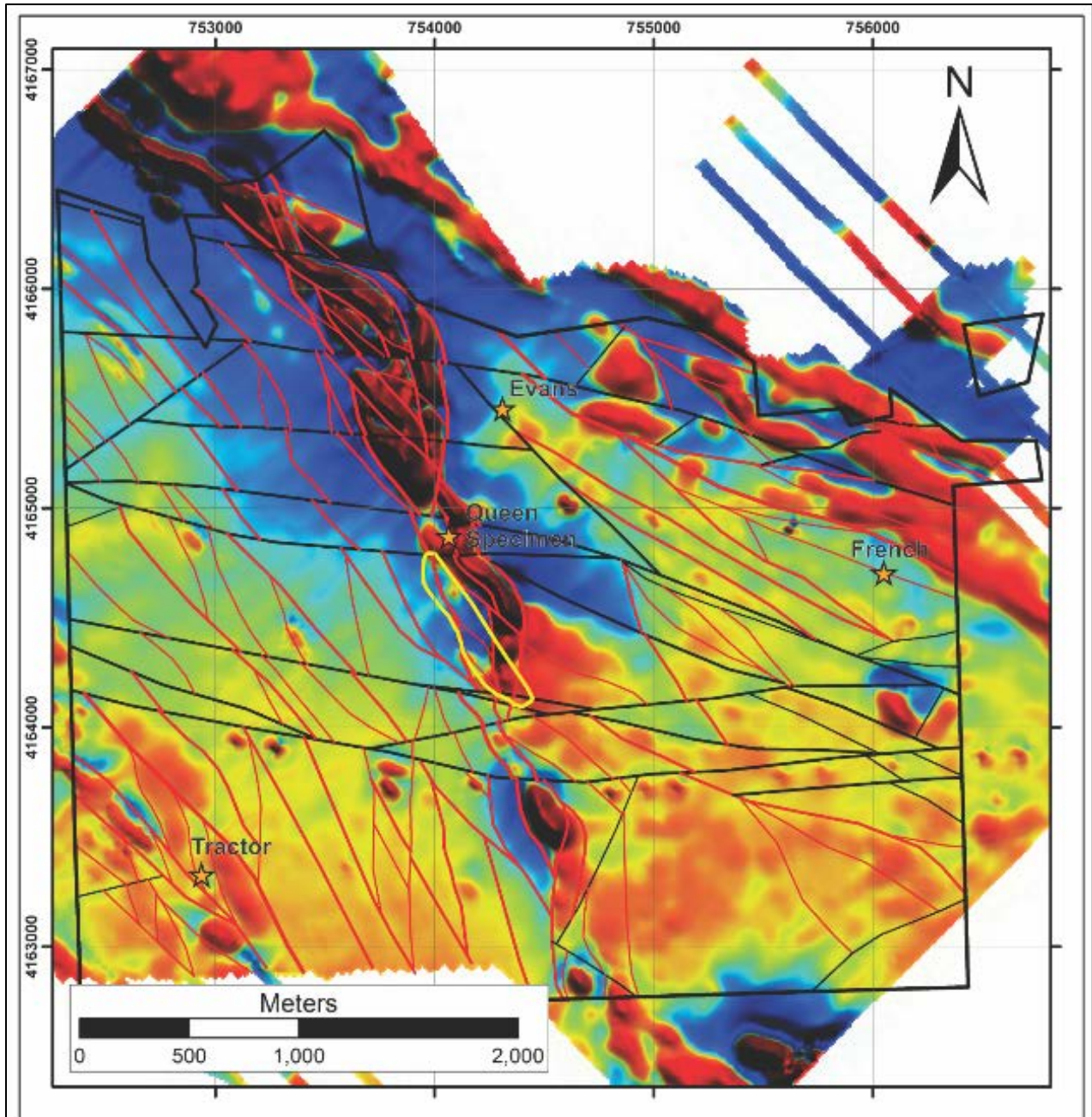
FIGURE 7.5 SRK STRUCTURAL INTERPRETATION OF MAGNETIC FIRST VERTICAL DERIVATIVE
